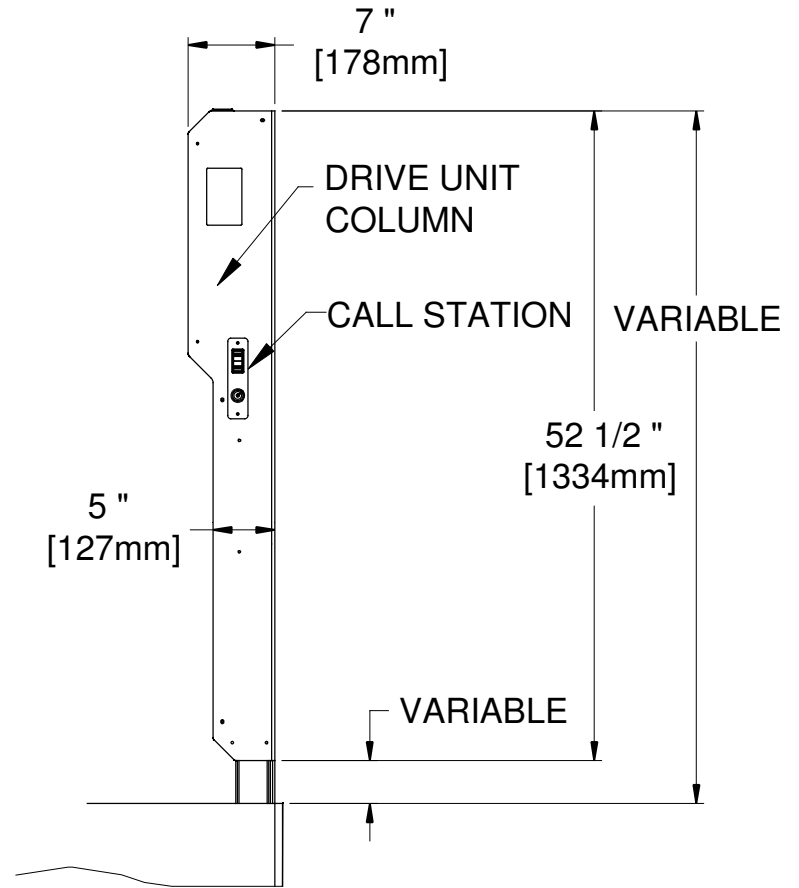
SIDE VIEW
