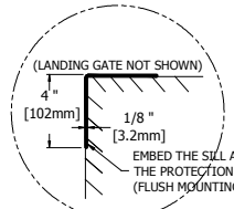
4 DETAIL C
