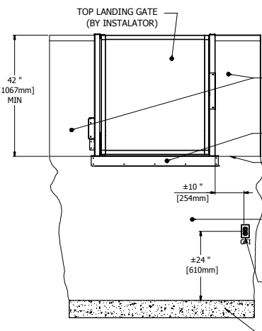
2 DETAIL A SIDE VIEW
