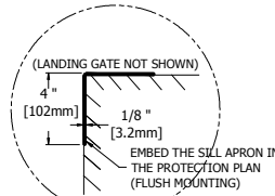
4 DETAIL C
